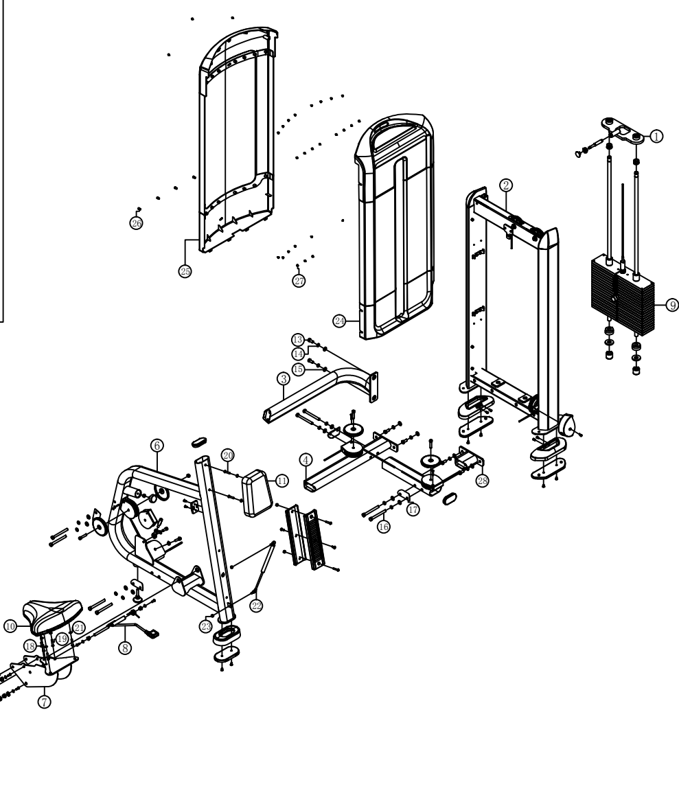
FF34 Seated row explosive view Note: spare parts and fasteners are not listed on the form.
