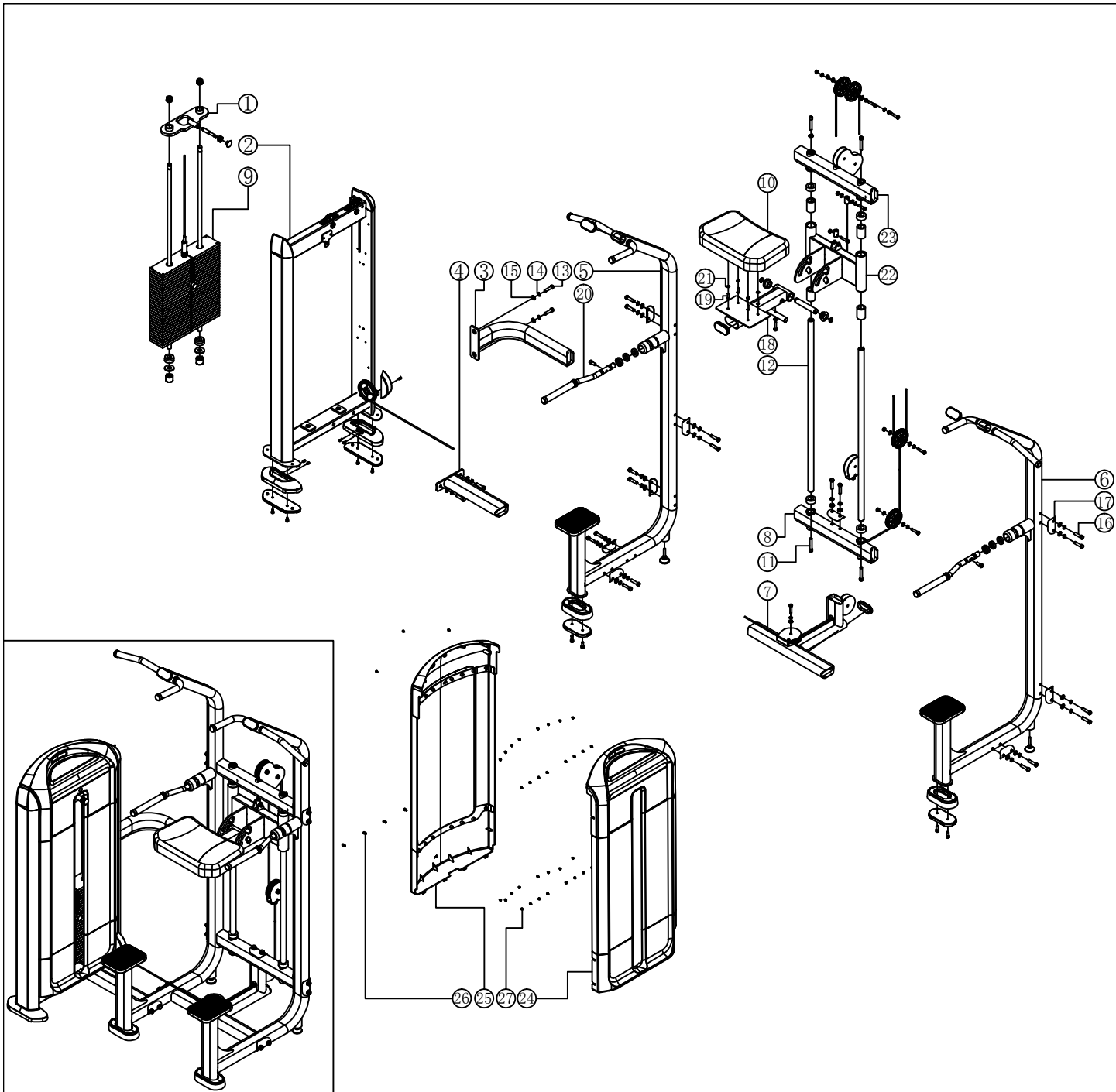
FF09 Diverging low row explosive view
